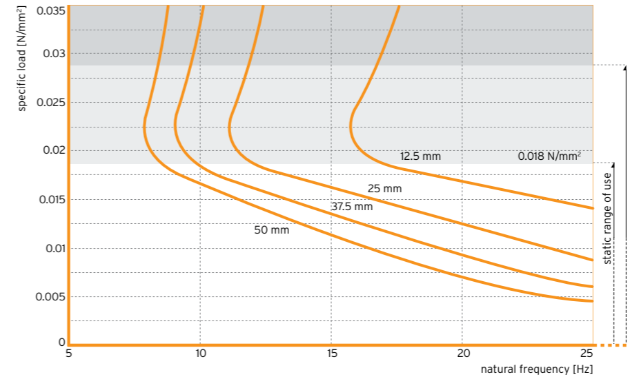
Figure 3: natural frequency of a single-degree-of-freedom system (SDOF system) consisting of a fixed mass and an elastic bearing consisting of Sylomer SR 18 based on a stiff subgrade;
