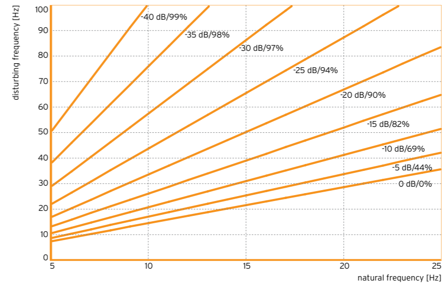
Figure 4: reduction of the transmitted mechanical vibrations by implementation of an elastic bearing consisting of Sylomer SR 18
